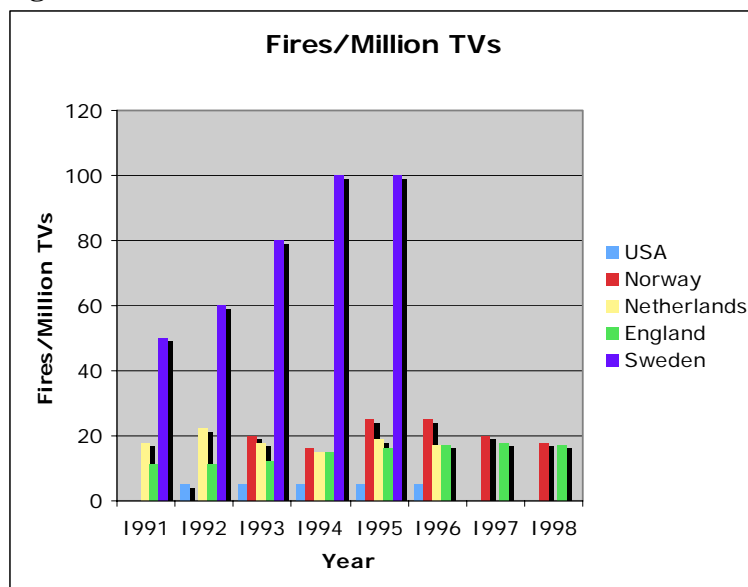
Figure 2. TV Fires/ million TVs
