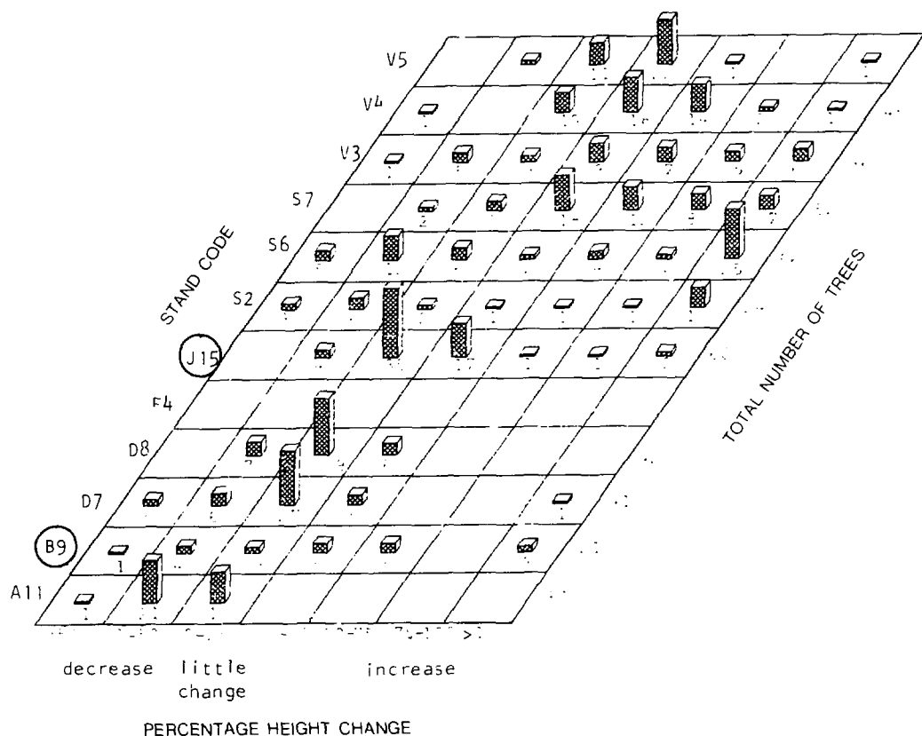
FIGURE 24 PERCENTAGE HEIGHT CHANGE IN ALL TREMBLING ASPEN STANDS. Trembling aspens on the Crotch site (Code S) exhibit definite height increases which are comparable to the control sites (J and B). The percentage change on the Bancroft sites is moderate.
