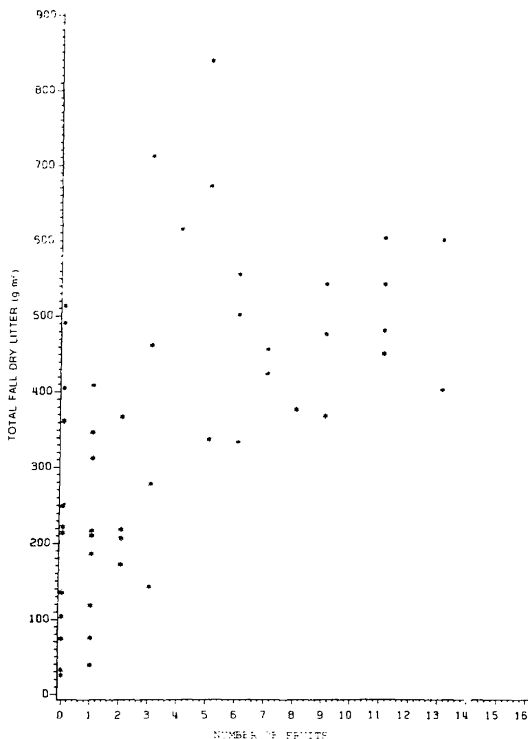
FIGURE 10 NUMBER OF FRUITS/ m^2 RELATED TO BIOMASS WEIGHTS/ m^2 FOR 1981. The relationship of above-ground biomass in g/m^2 and the number of fruit bearing shoots is presented for 37 quadrats with a correlation coefficient of 0.49 (significant at p < 0.01 ) which explains 25 percent of the variation between the two variables.
