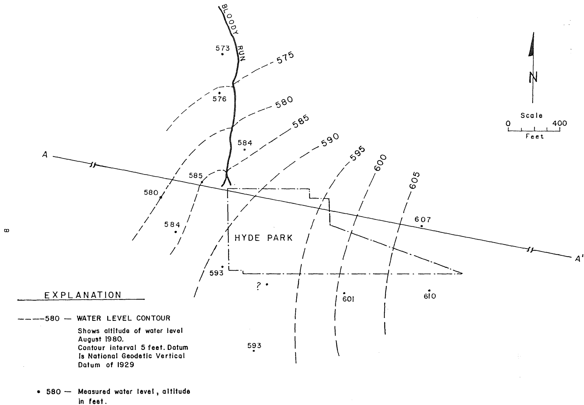
Figure 3 -- Ground-water levels in the uppermost part of the Lockport Dolomite near Hyde Park landfill, August, 1980.
