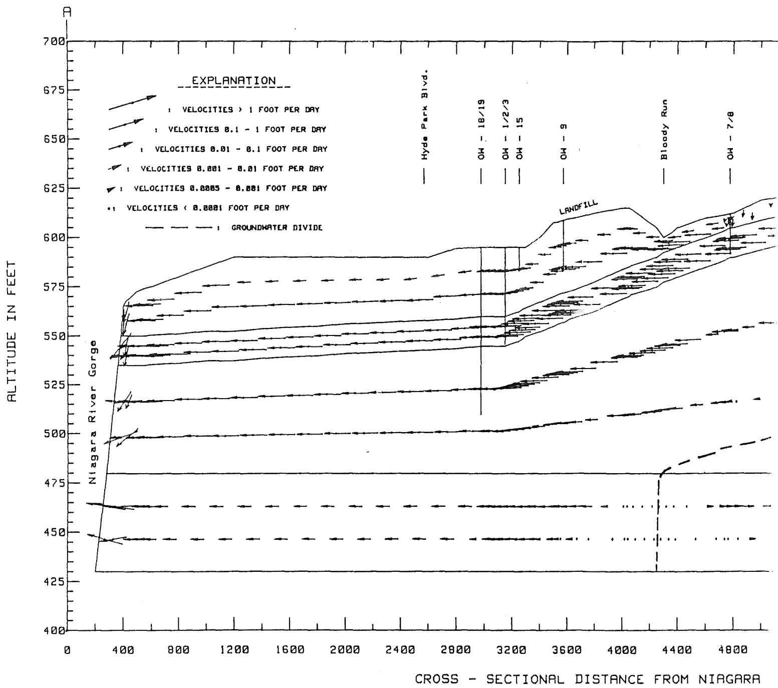
Figure 6. -- Elemental Darcy Velocity
