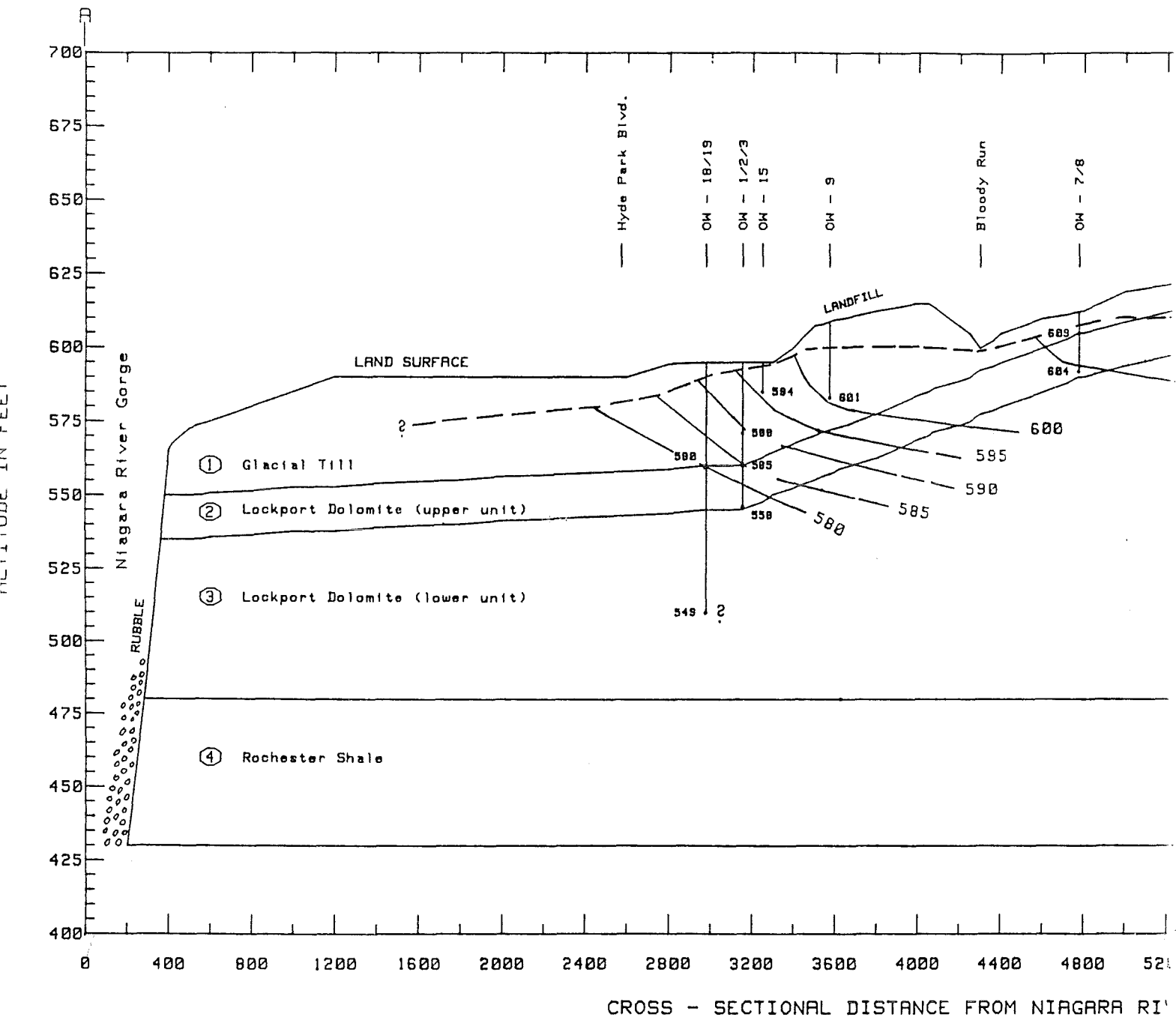
Figure 2. -- Hydrogeologic units, depth and location of and average 1980 ground-water levels
