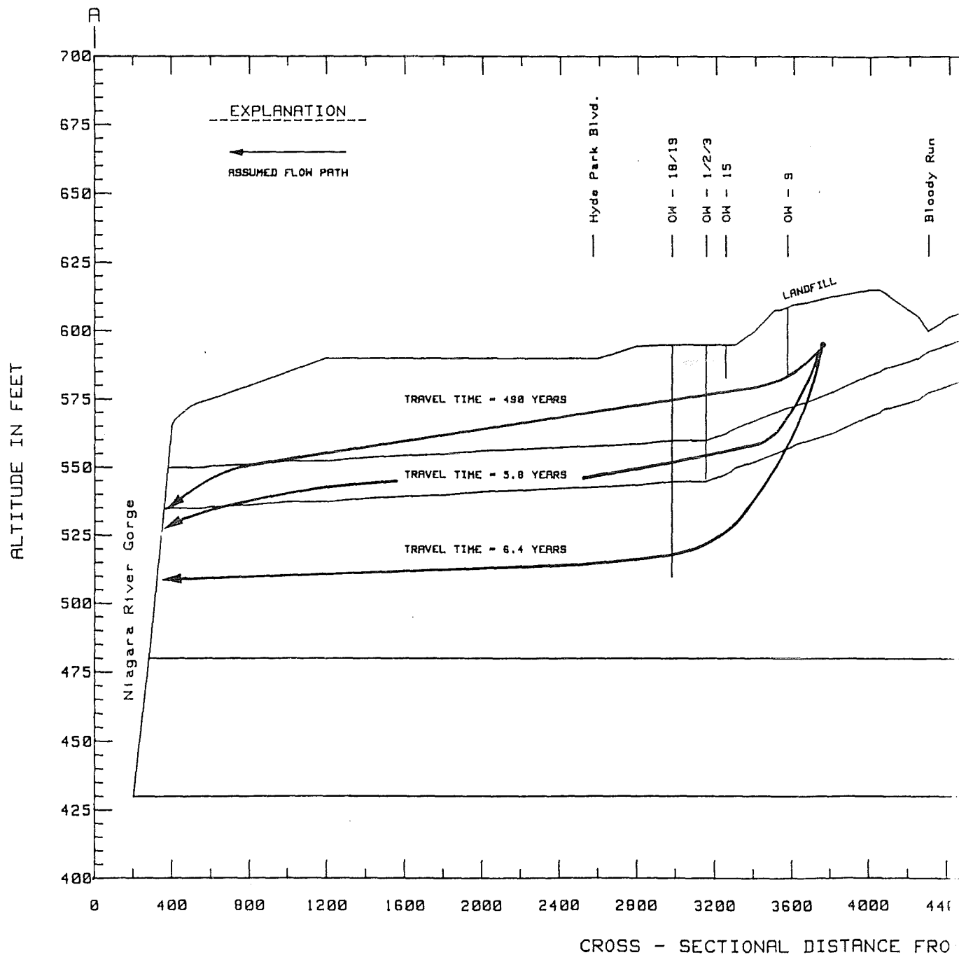
Figure 7. -- Estimated time of travel for ground water
