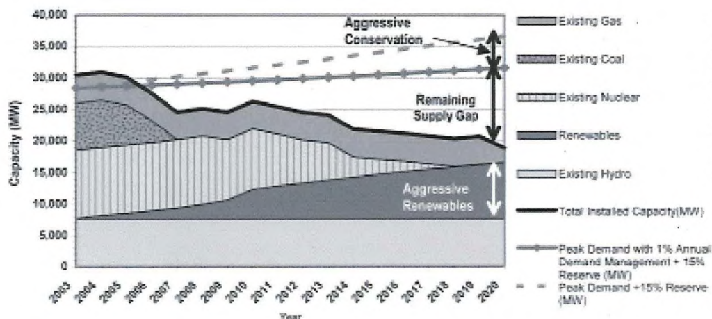
Figure 1: Electricity Supply and Conservation Task Force Projection of Generation vs. Peak Demand— With Renewables
