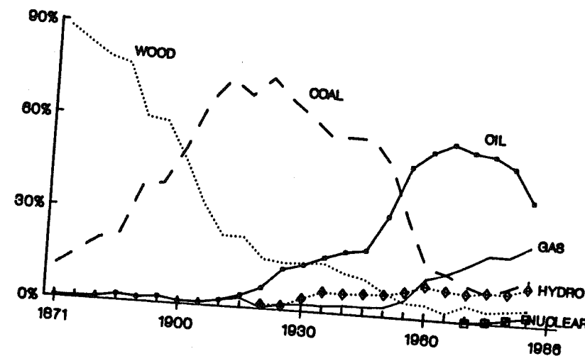
Figure 1.1 PRIMARY ENERGY BY SOURCE, CANADA 1870 - 1986
