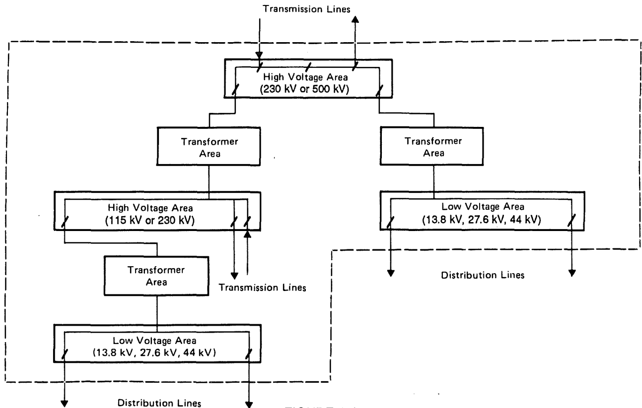
FIGURE 4-4 Components of a Typical Transformer Station – Complex
