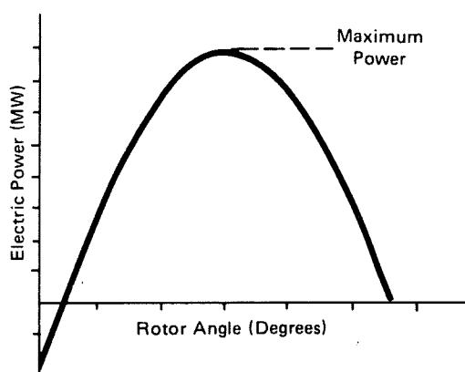
FIGURE E-2 Power Angle Relationship of a Synchronous Generator
