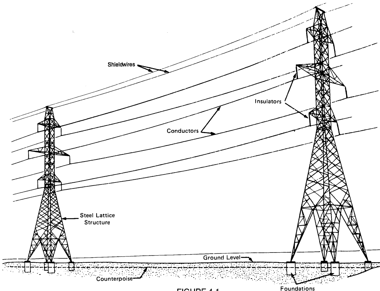
FIGURE 4-1 Component Parts of a Typical Transmission Line
