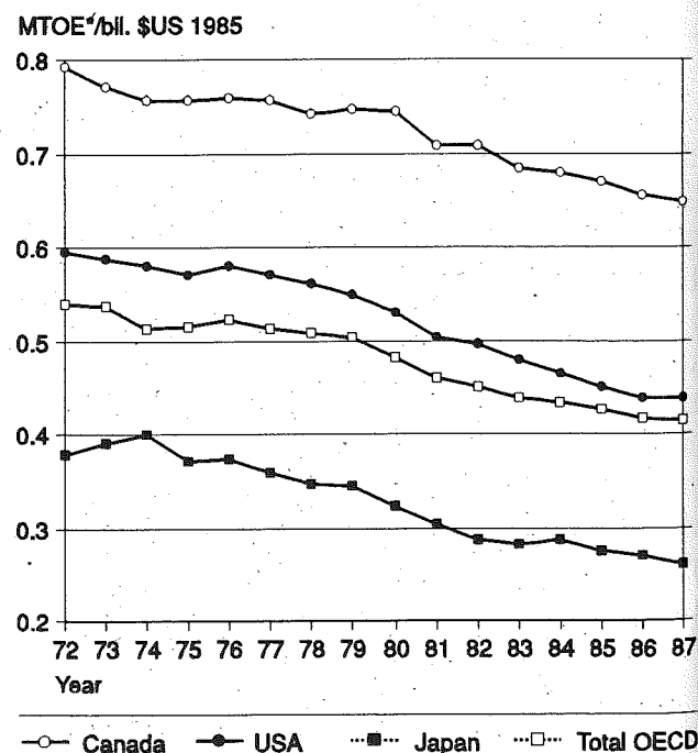
Figure 26. Primary Energy Use Per Unit of GDP
