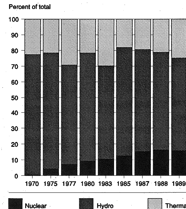
Figure 25. Electrical Generating Capacity by Type
